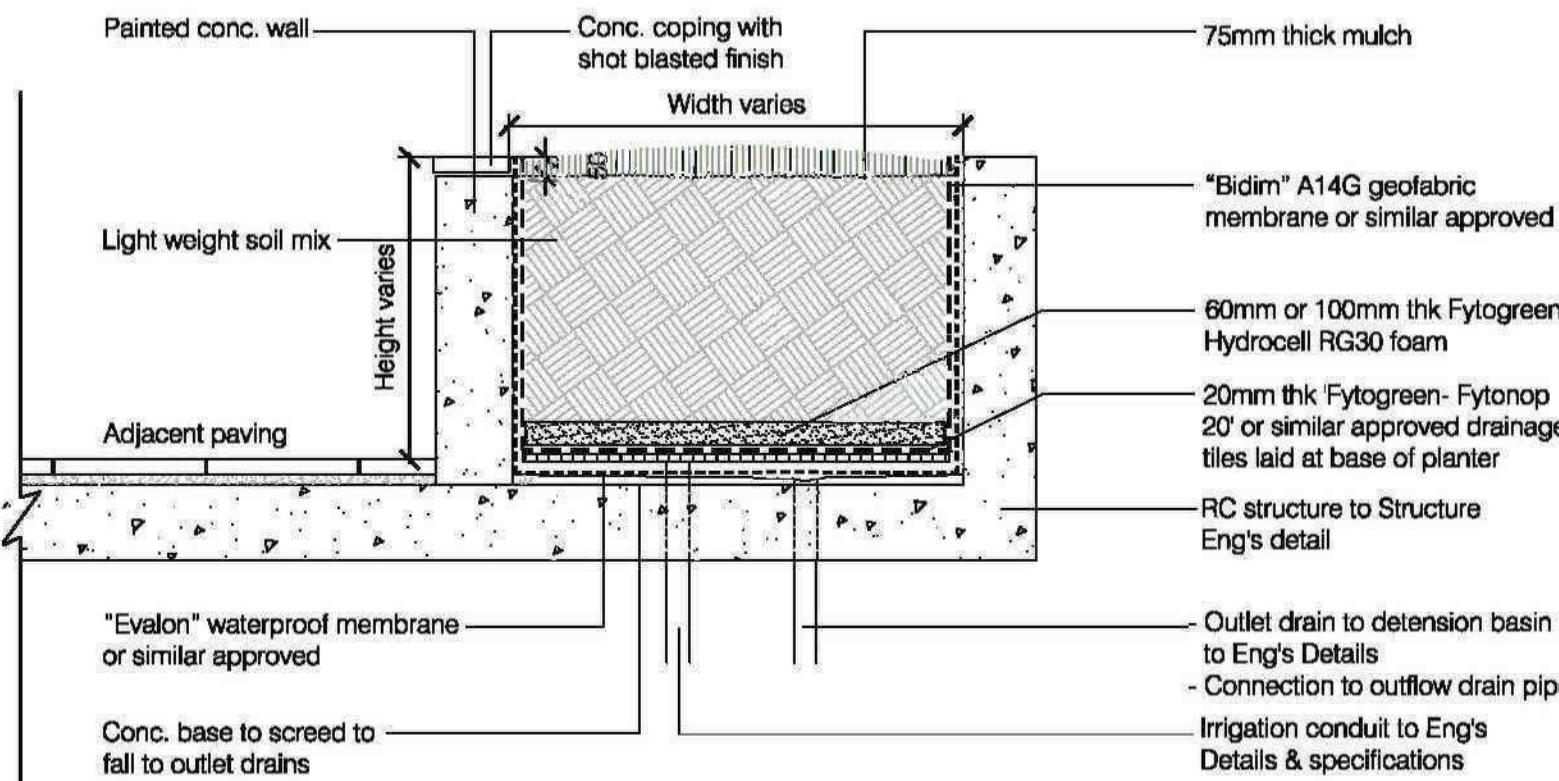
TYPICAL DETAIL 04: on-structure planter scale: 1:20
